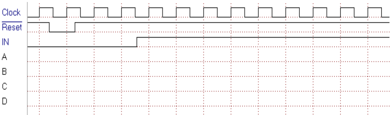
Timing Sequence (A):
