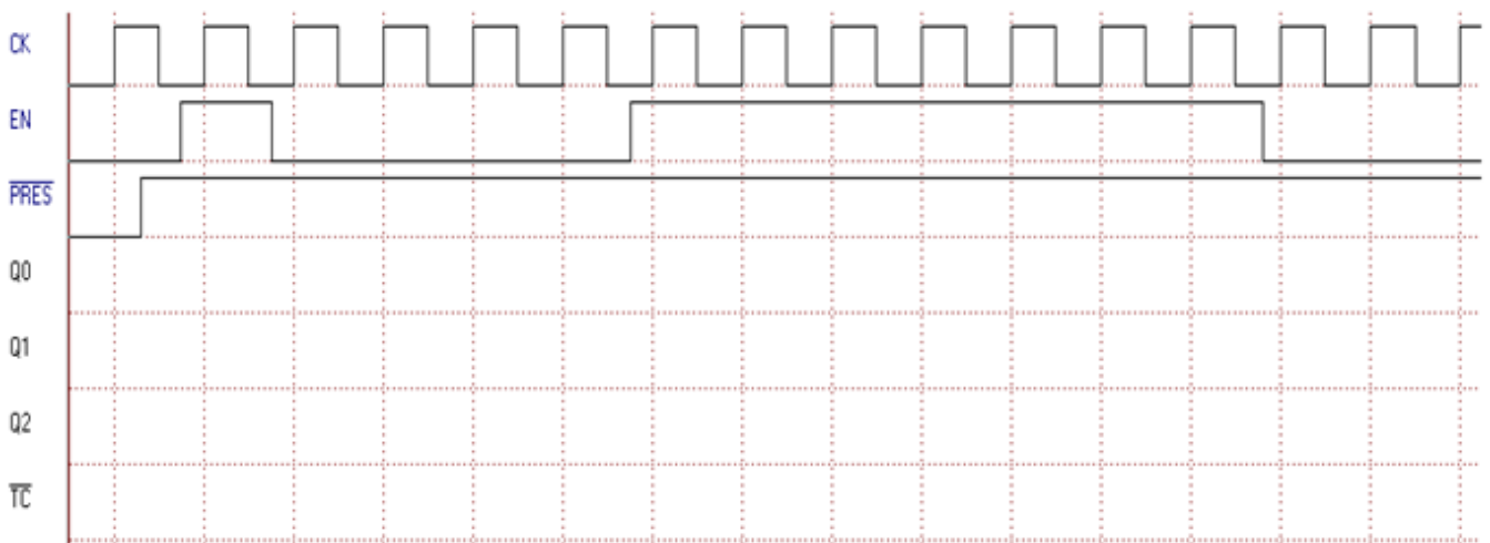
Timing Sequence (B)
