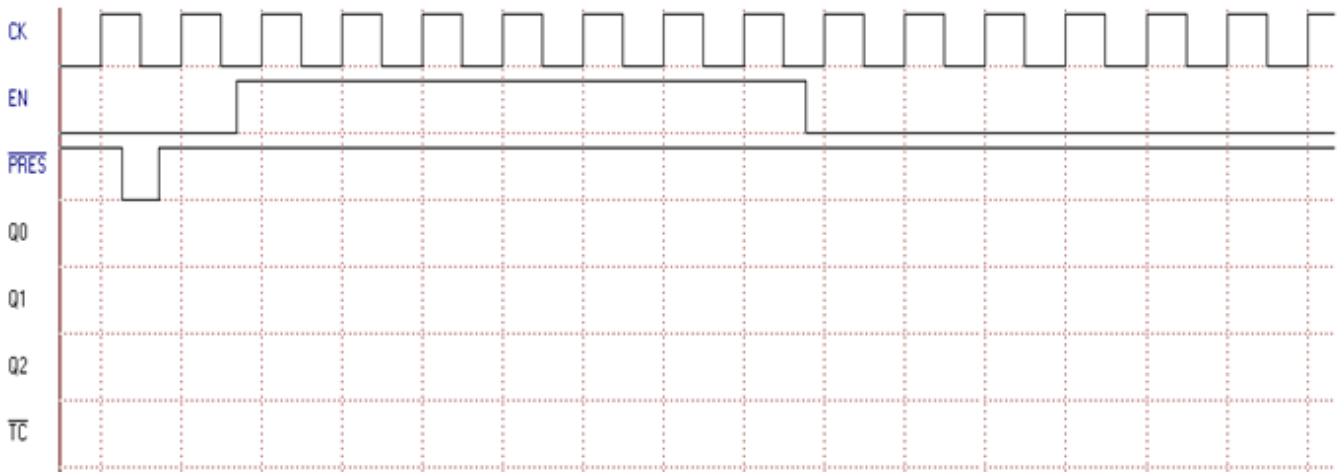
Timing Sequence (A):
